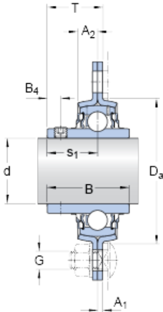
PFT 1.1/4 TR Bearing 2D drawings and 3D CAD models
